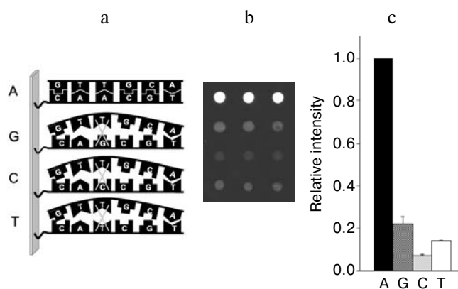
Fig. 5. a) Scheme of point mutation detection in gene by allele-specific hybridization. b) The result of point mutation detection in a gene by hybridization analysis on microchip. c) Representation of results of hybridization analysis for detection of a single mutation in a gene in relative units.
