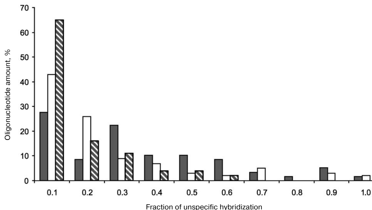
Fig. 7. Relative specificity of point mutation detection in CTX-M type beta-lactamase genes by hybridization analysis on microarrays with fluorescence and colorimetric detection. Black columns: Cy3 DNA label, hybridization conditions 45°C, 1 h; white columns: Cy3 DNA label, hybridization conditions 47°C, 1 h; hatched columns: biotin label, hybridization conditions 45°C, 2 h.
